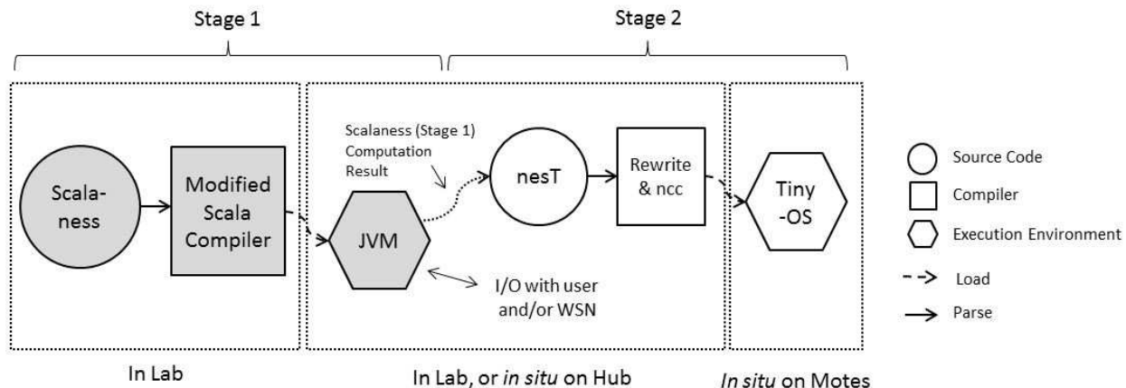
Figure 1. Scalanness/nest Compilation and Execution Model
