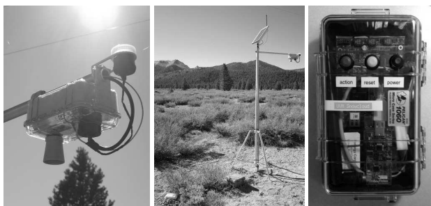
Figure 2. A Sensor Node (L,C) and Hub Device (R).
